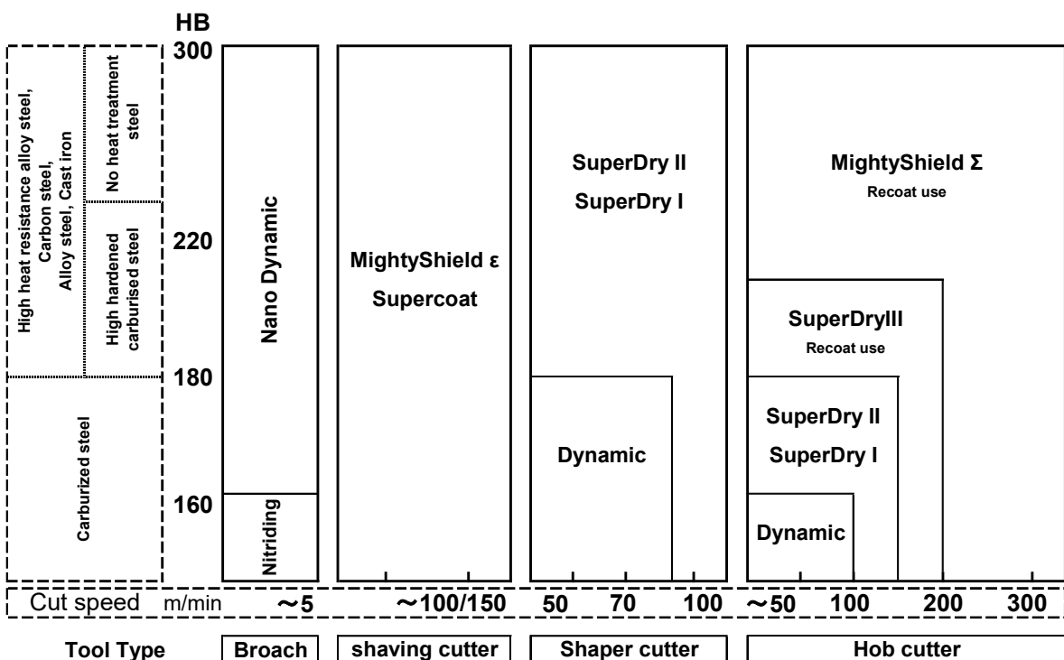
Surface treatment selection map
