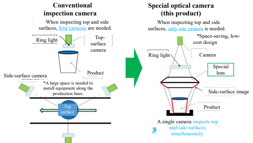
Nidec Tosok's Actual-bottle visual inspection equipment
