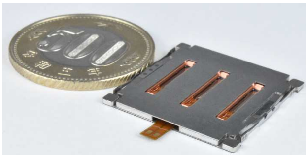
“TapSense”
